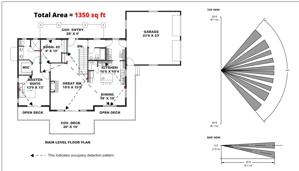
Figure 9. Occupancy Sensor Detection Pattern Examples
